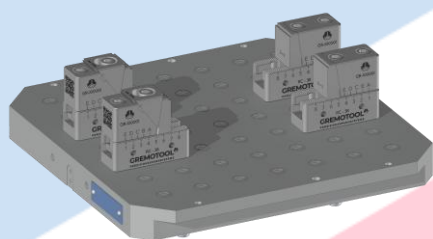
2x RC-38 & System 3R Delphin 398 Pallet
