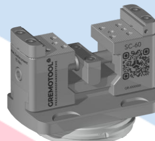
SC-60 & System 3R GPS-120 Pallet
