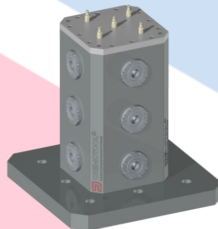
8x SC-40 con Torre & System 3R Delphin 398 Pallet
