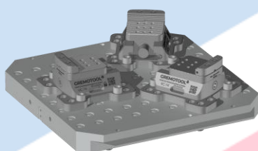
3x VC-74 & System 3R Delphin 398 Pallet
