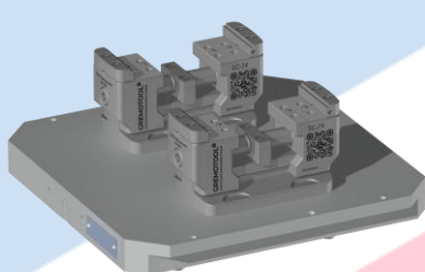
2x SC-74 & System 3R Delphin 398 Pallet
