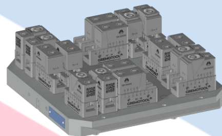
8x RC-38 & System 3R Delphin 398 Pallet
