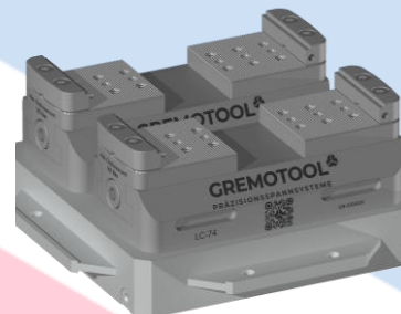
2x LC-74 & System 3R GPS-240 Pallet
