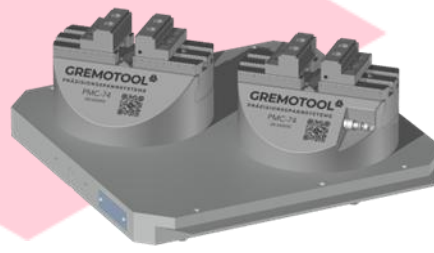
2x PMC-74 & System 3R Delphin 448 Pallet
