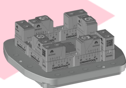
4x RC-38 & System 3R Dynafix Pallet
