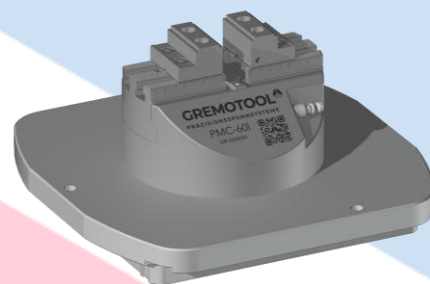
PMC-60I & System 3R Dynafix Pallet
